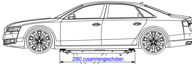
Audi A8, Langversion (2014) 1:30 L: 5.265 B: 1.949 H: 1.460 R: 3.122
